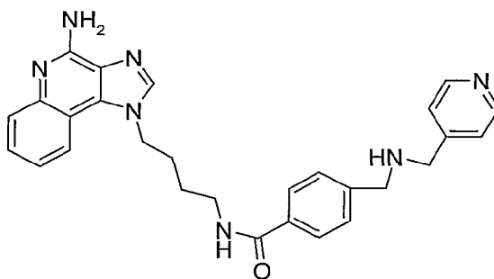
N -[4-(4-amino-1 H -imidazo[4,5- c ]quinolin-1-yl)butyl]-4-[(pyridin-4-ylmethyl)amino]methylbenzamide;
